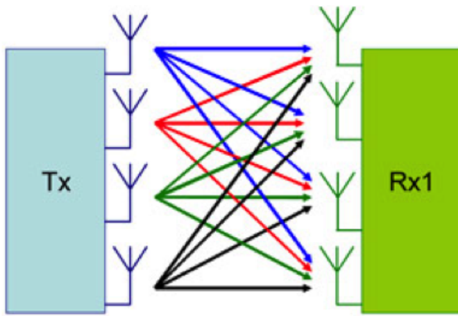
(a) Single User MIMO, 4 streams
